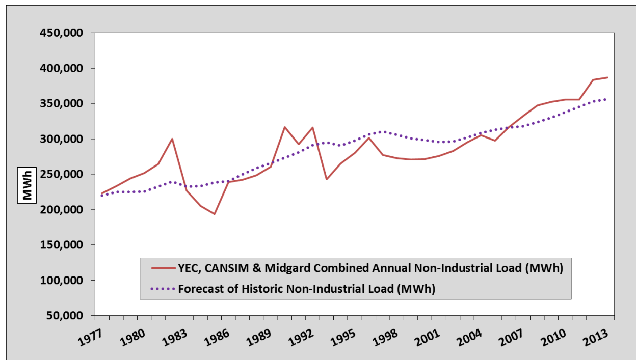
Figure 3-8: Historic Non-Industrial Electrical Energy Demand & Forecast of Historic Non-Industrial Electrical Energy Demand
