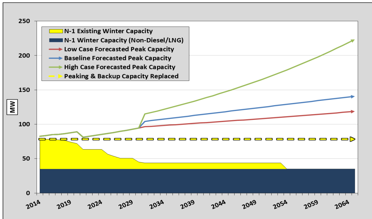
Figure 4-6: High, Baseline & Low Case Electrical Capacity Demand & Electrical Supply Capacity (2014 - 2065)
